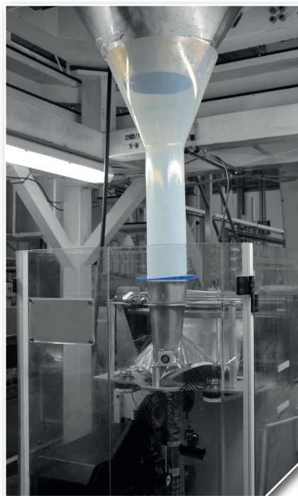
Versa-chute® Bag Maker Chute (3mm)
